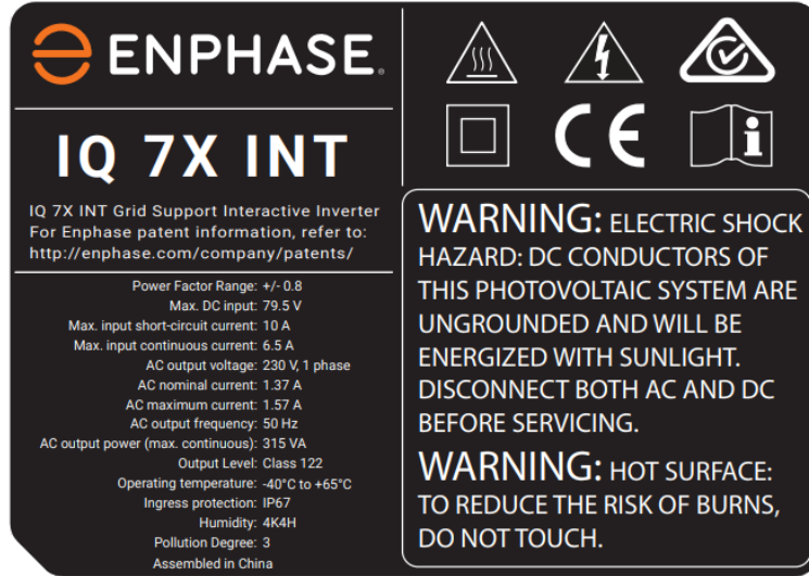
Figure 1: IQ7X marking plate
